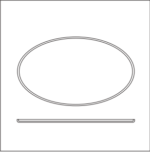
OVAL TRAY 272x191x12mm
