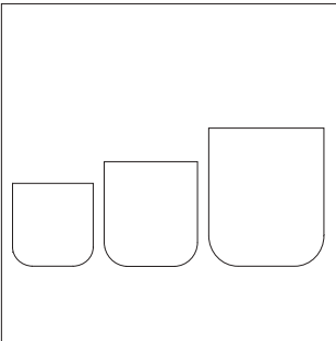
CAPSULE CUP S, M, L S: 70x72 mm M:81x91mm L: 100x120mm
