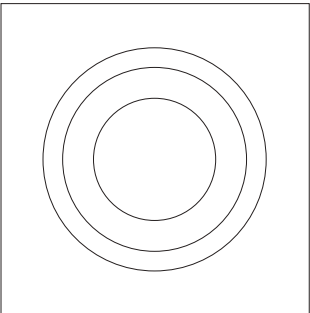
PLACEMAT ROUND S, M, L S: Ø196mm M: Ø295mm L: Ø358mm
