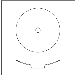
BASIN 403x75mm, Ø403mm, hole 42mm
